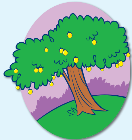
Tree Of Life
